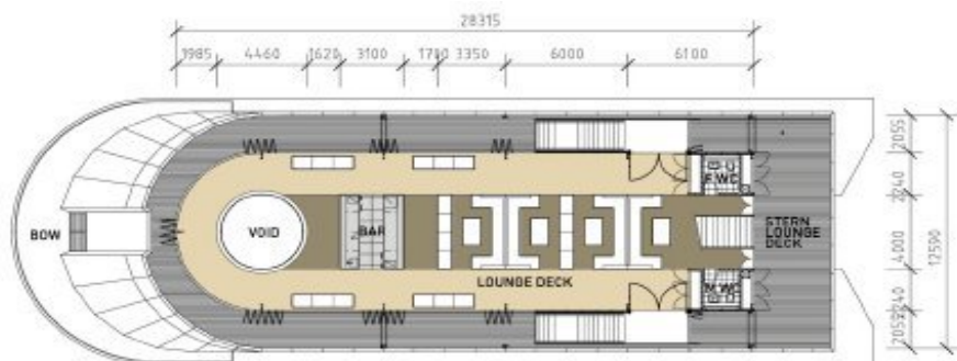
1 LOUNGE DECK
