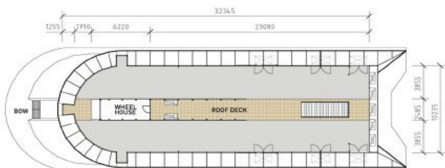
2 ROOF DECK
